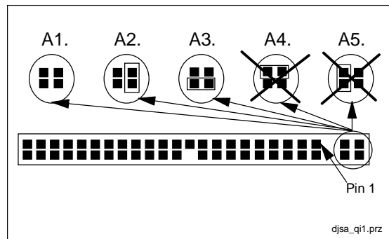
Jumper settings
